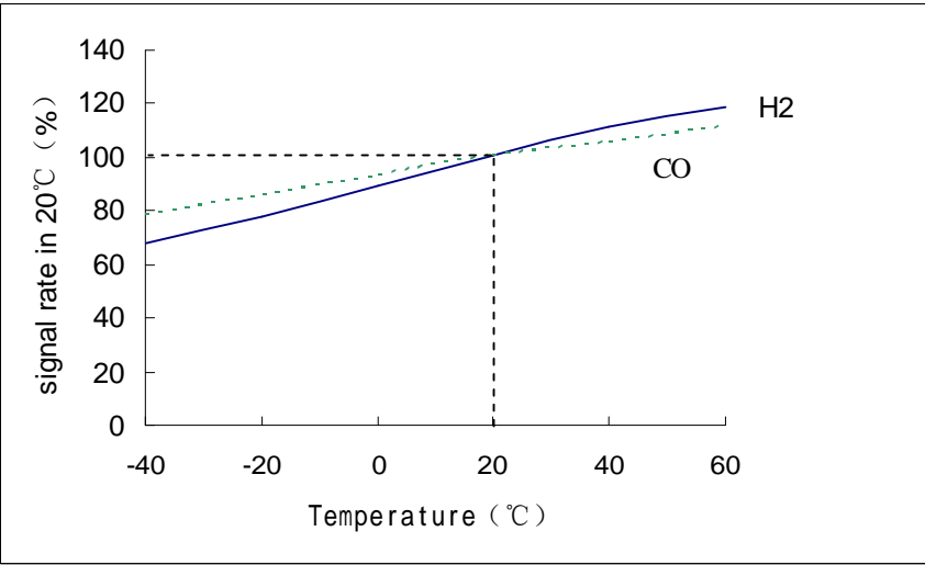
Chart 4. Temperature curve
